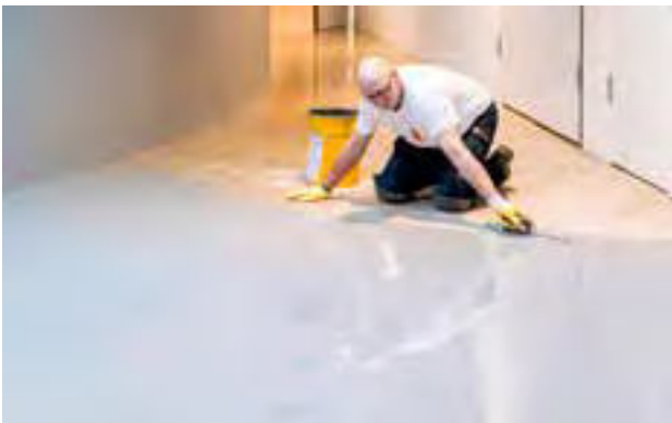
STEP 3. Self-leveling materials are applied in one or several layers to create a seamless base. Experts will pour and distribute the liquid material by using special squeegees, hand trowels, stand-up trowels and spike rollers in the process to assure a perfectly even and smooth surface.
