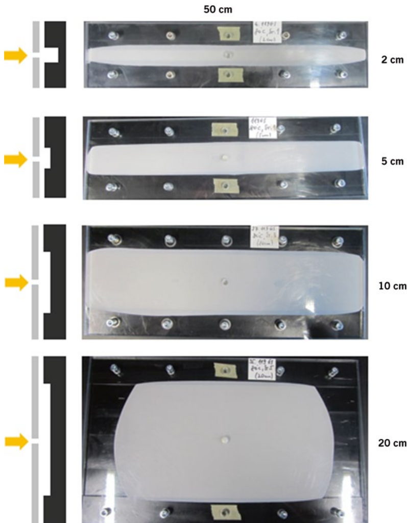
FIGURE 5 Injection into various channel widths (© Sika)
