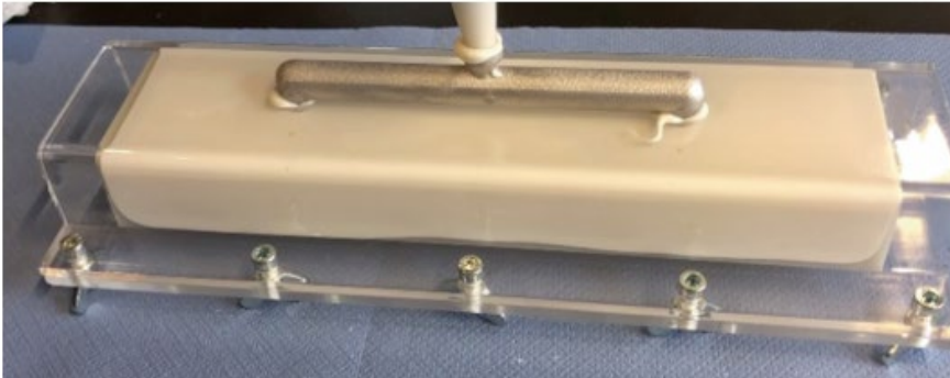
FIGURE 7 Multiple injections with SikaPower Standard (top) and SikaPower SmartFlow (down) (© Sika)
