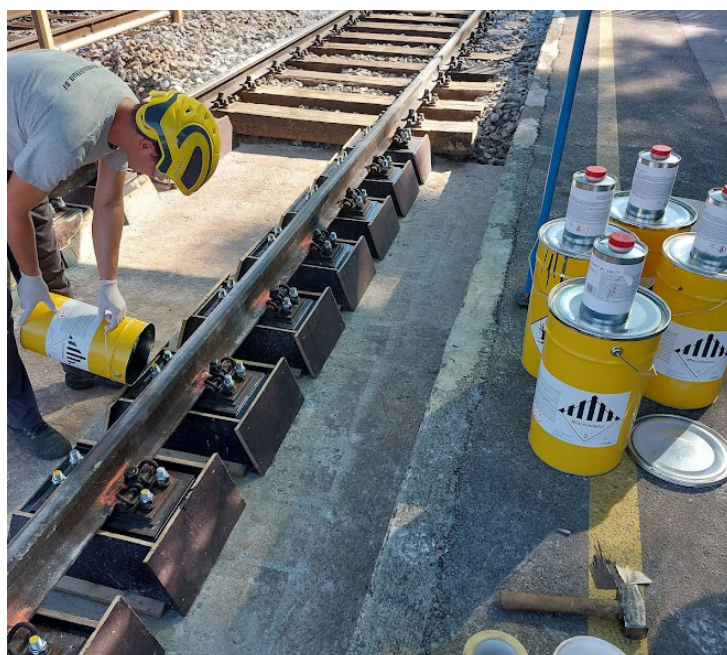
Installation of Icosit® KC 340/7 material.
